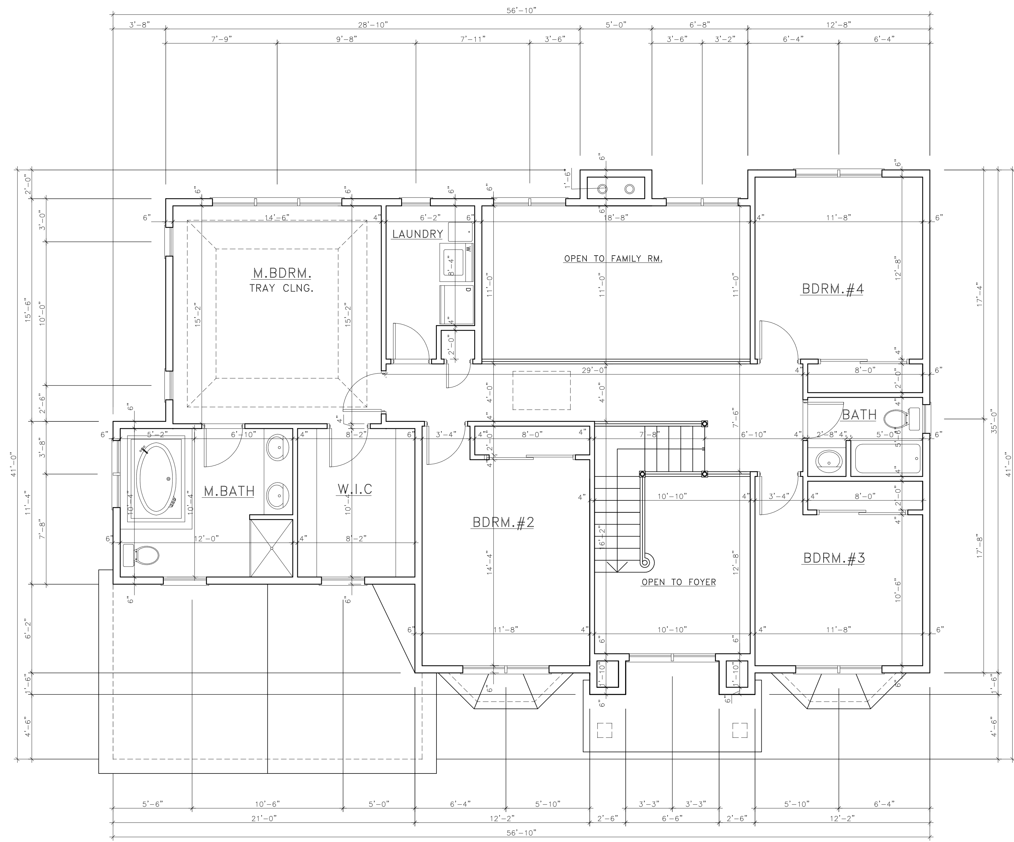
1 SECOND FLOOR PLAN A-5
