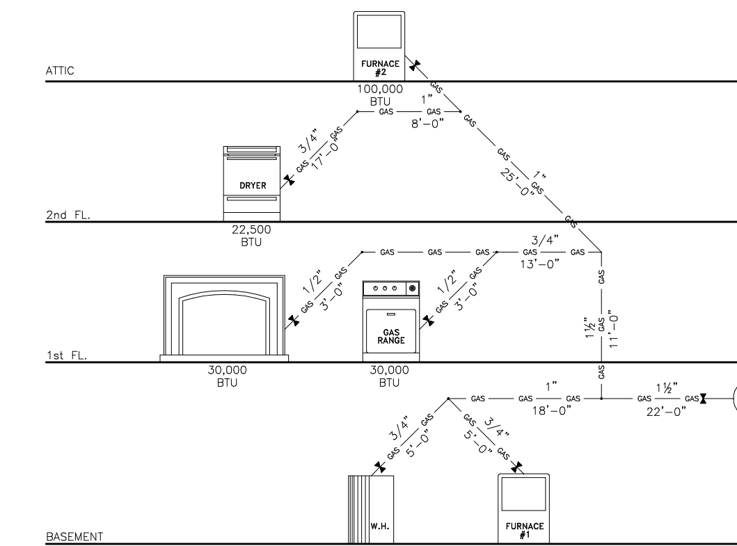
3 GAS RISER DIAGRAM A-3
