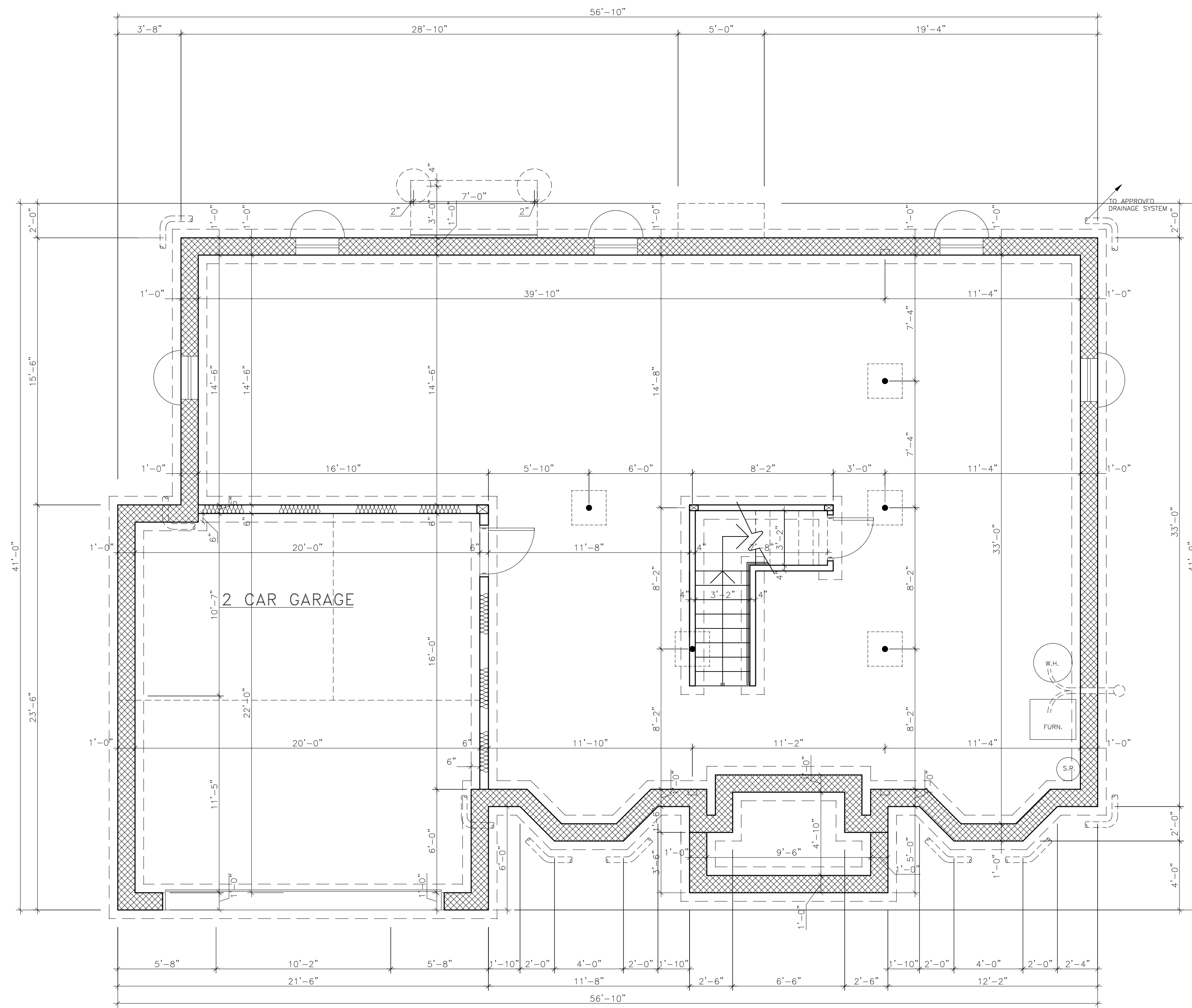
1 BASEMENT/FOUNDATION PLAN A-3
