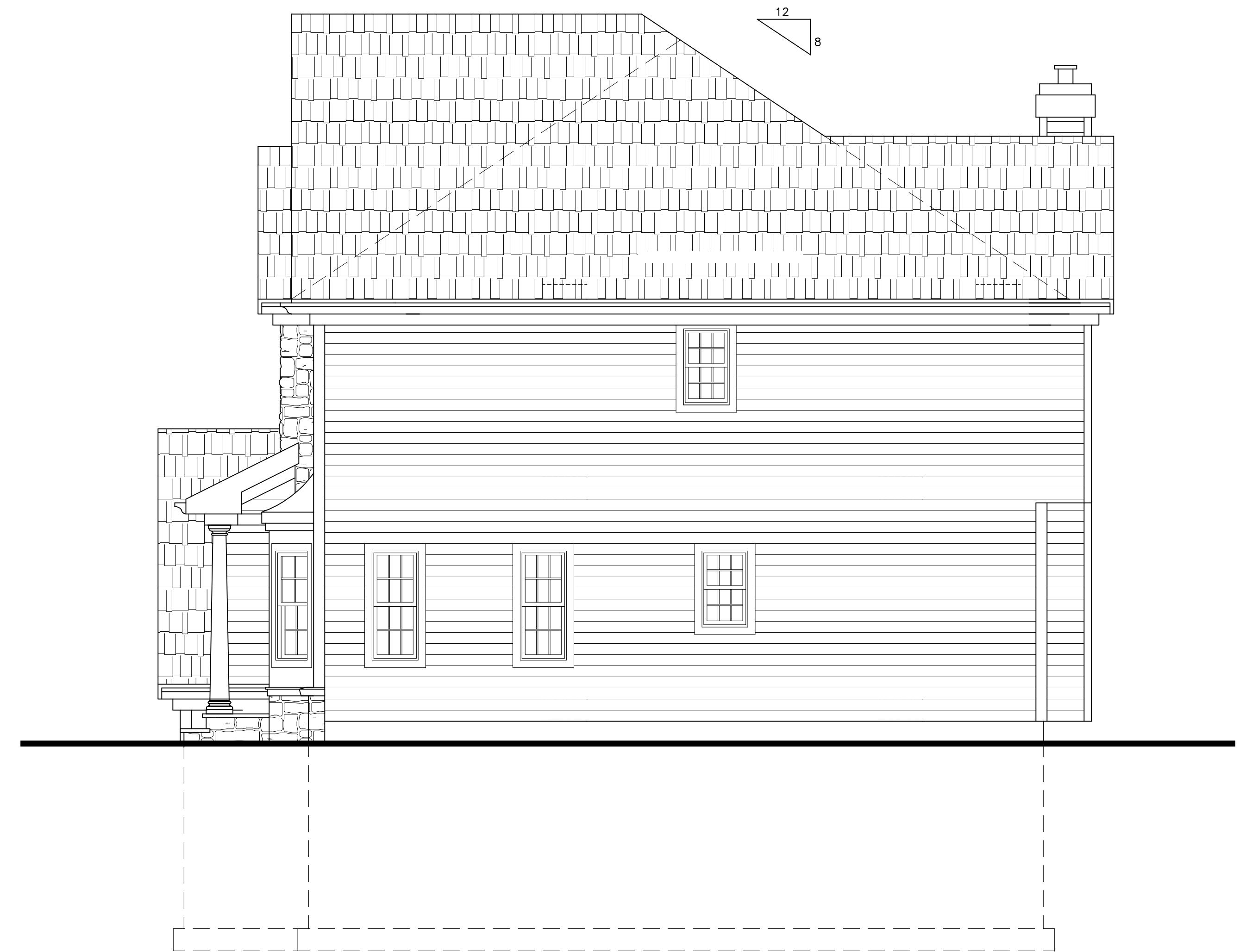
2 RIGHT SIDE ELEVATION A-2 SCALE 1/4"=1'-0"
