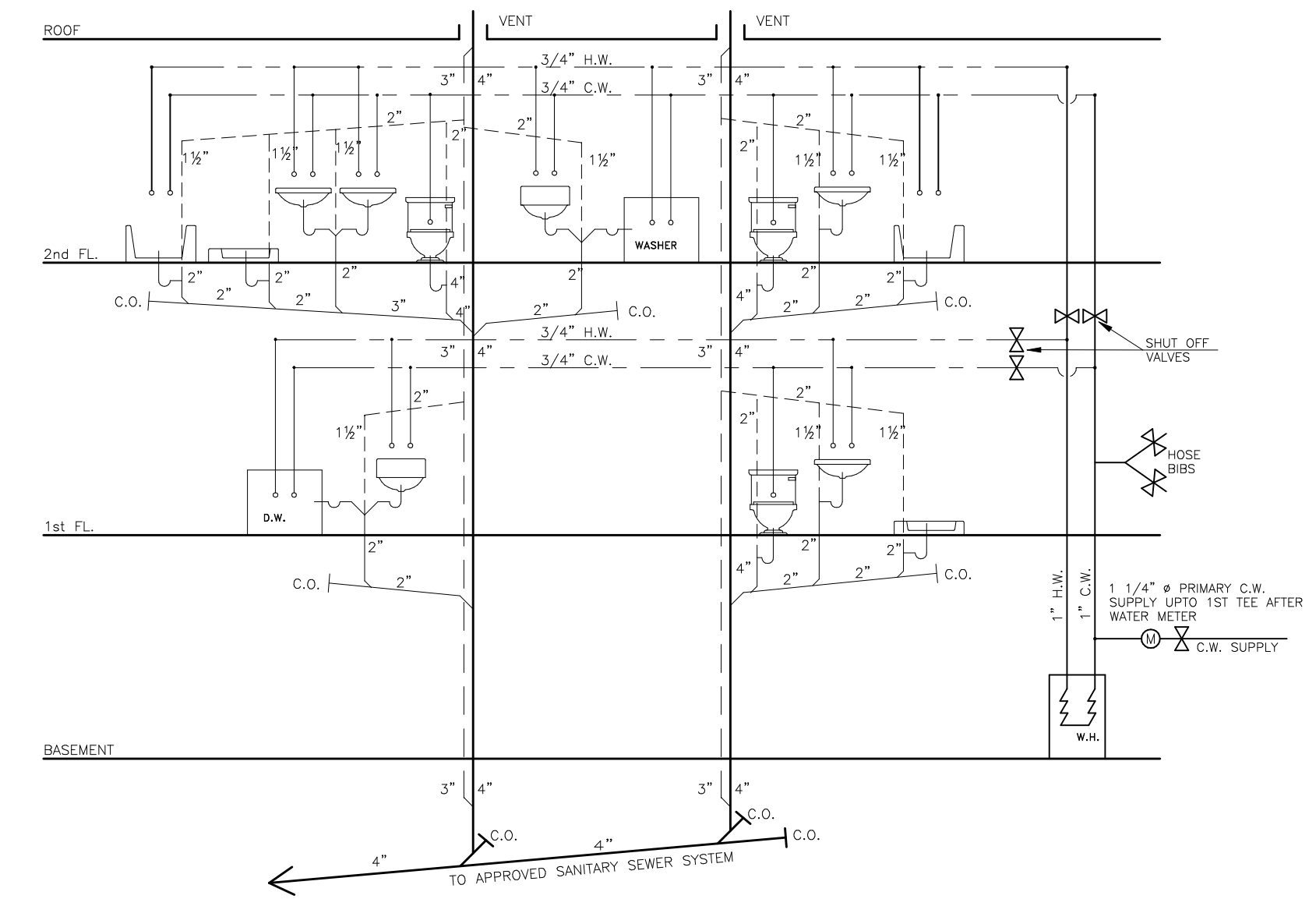
2 PLUMBING RISER DIAGRAM A-3
