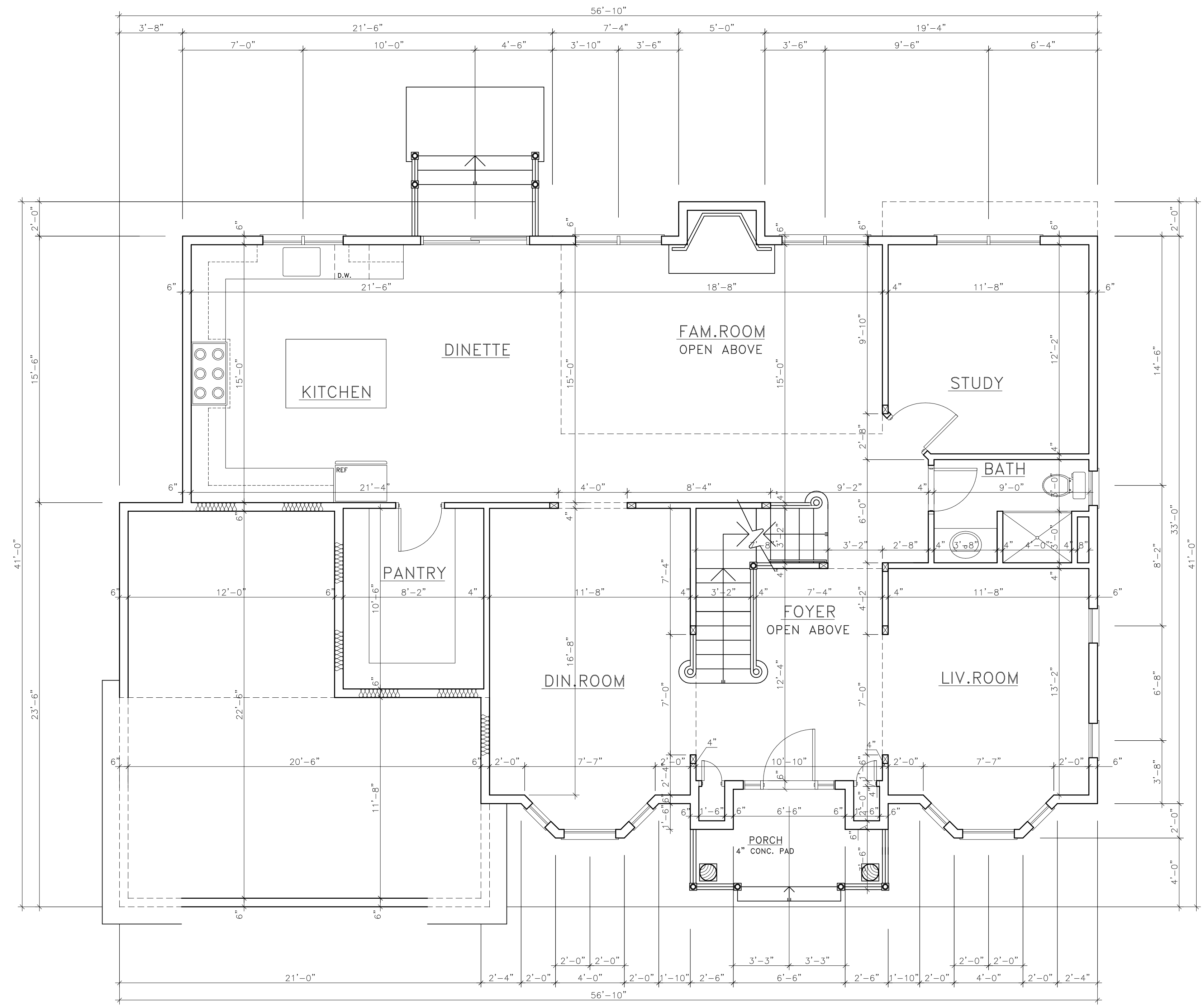
1 FIRST FLOOR PLAN A-4 SCALE 1/4"=1'-0" AREA - 1577.00 S.F. VOLUME - 15770.00 C.F.
